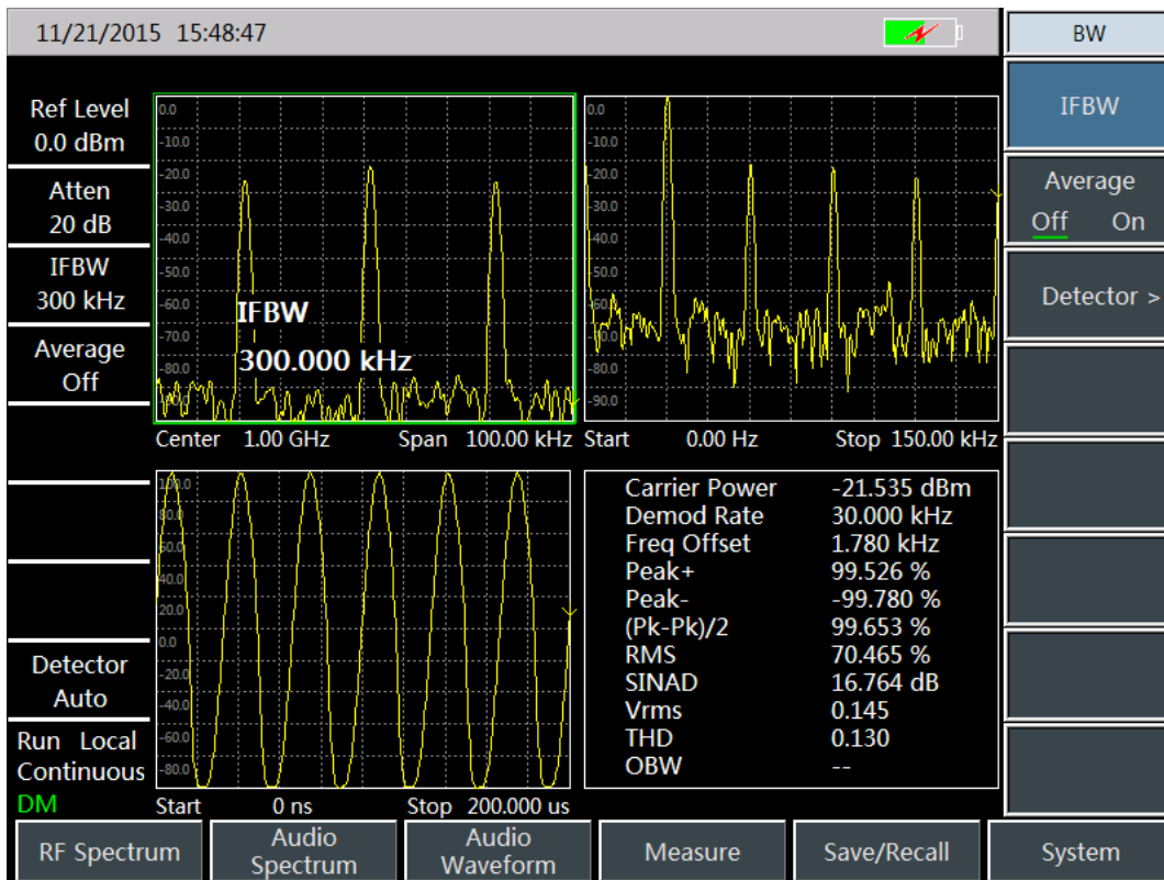
AM/FM/PM demodulation
