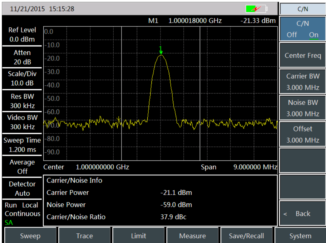
Carrier-to-noise ratio
