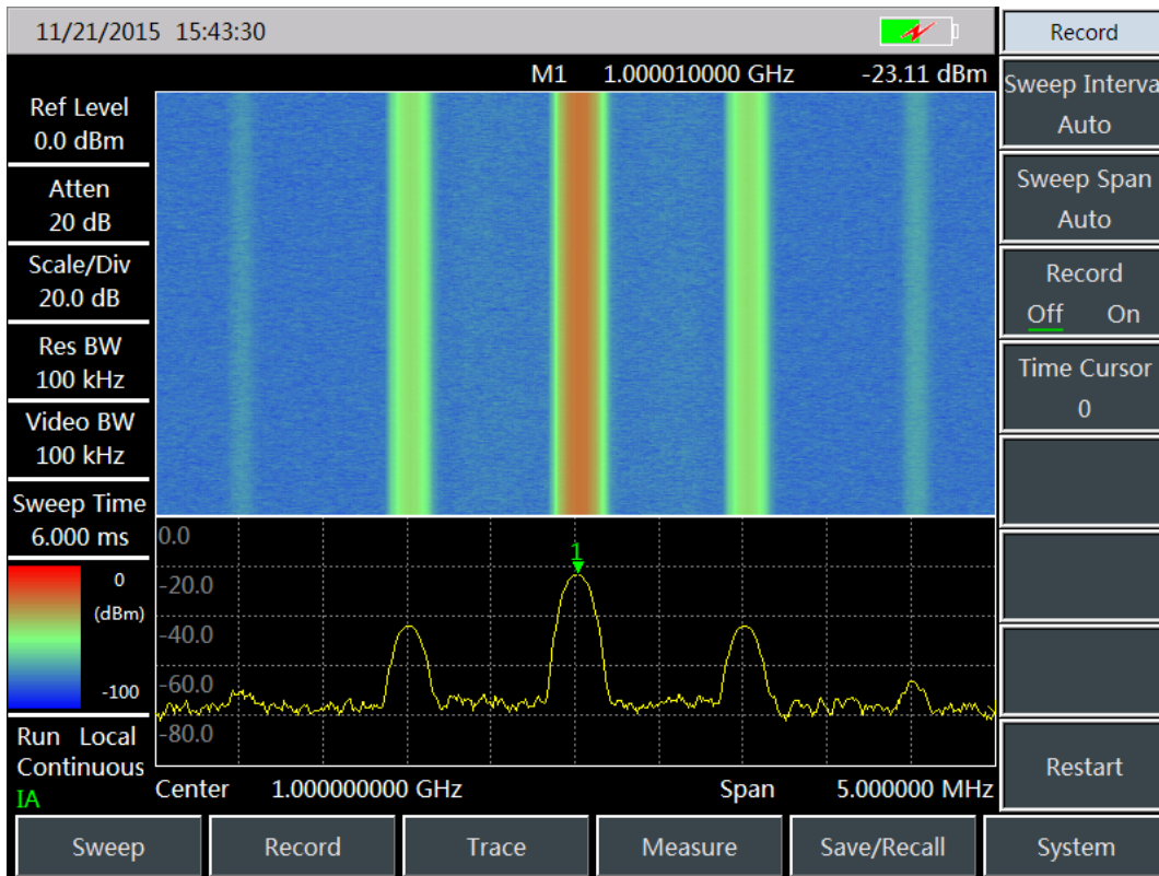
Interference analyzer (waterfall diagram)
